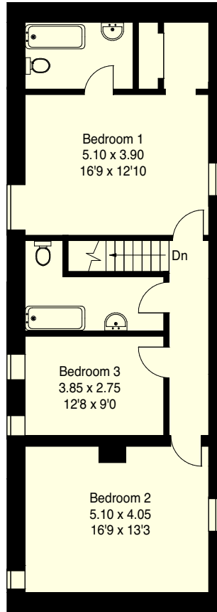
First Floor
